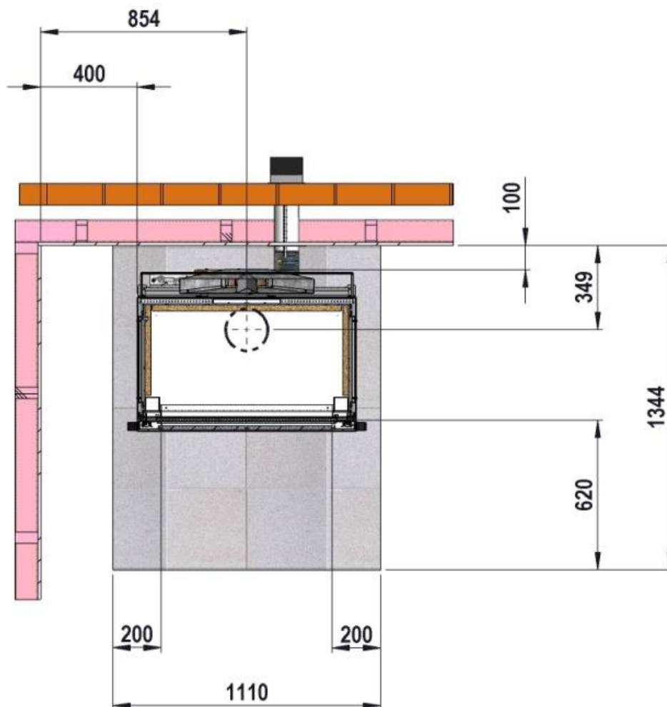
Fig 1 – Plan View - Tommi Installed Parallel to Main Wall
