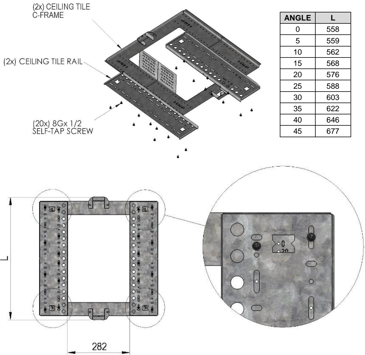
Fig 4 – Sloped Ceiling - Angles
