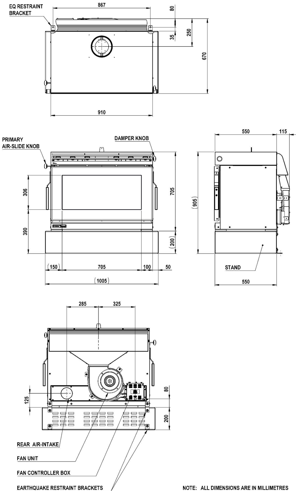
FIG. A: HEATER DIMENSIONS – TOMMI WOODBURNER (Not to Scale.)
