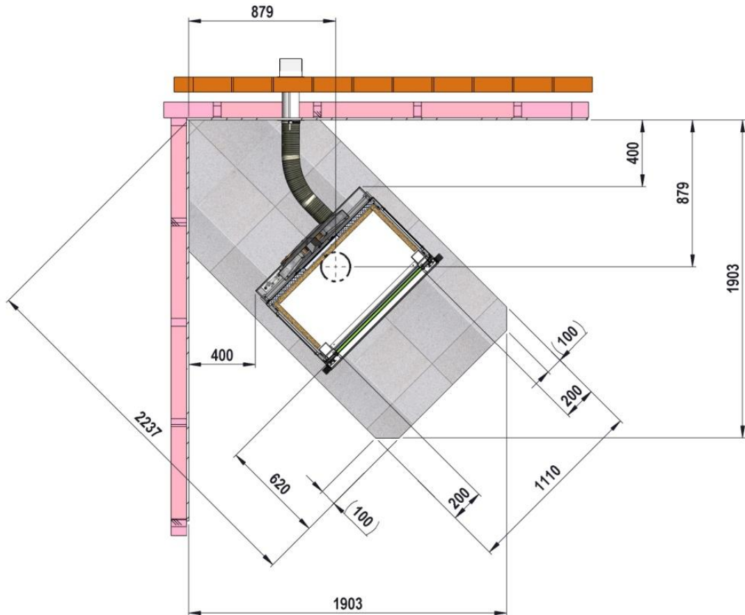
Fig 2 – Plan View – Tommi Installed Diagonally
